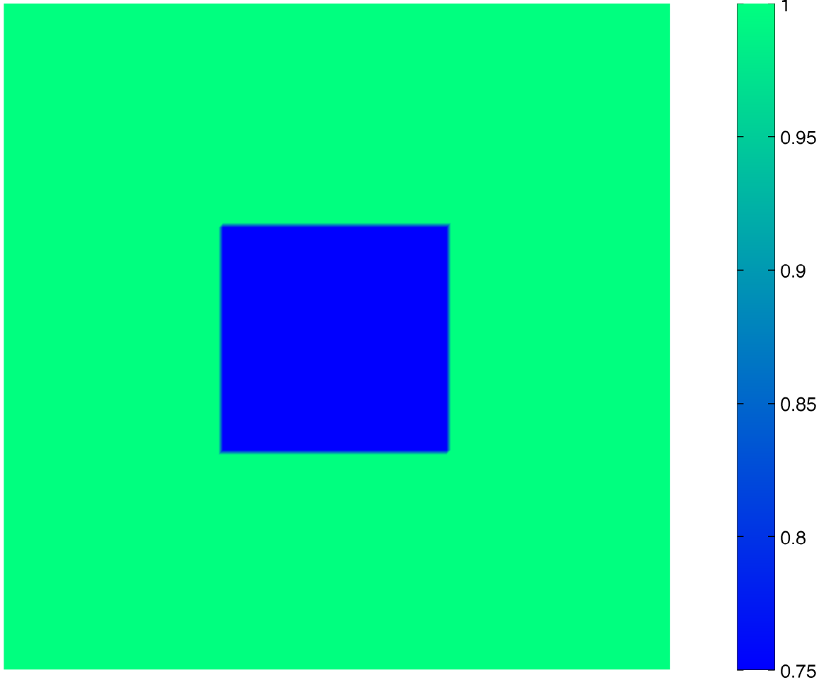
Solution at t = 0 (First component)
