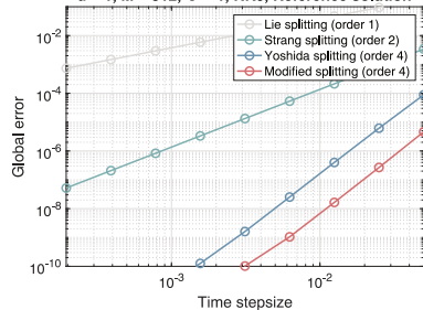
Schroedinger equation, Quadratic potential d = 1, M = 512, \vartheta = 1, \text{RK0, Reference solution}
